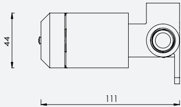
MW13BDY Wall Mixer Concealed Body • Used together with any MW03 finish set • Flow rate 18 litres per minute • European components and cartridge • Solid brass construction
